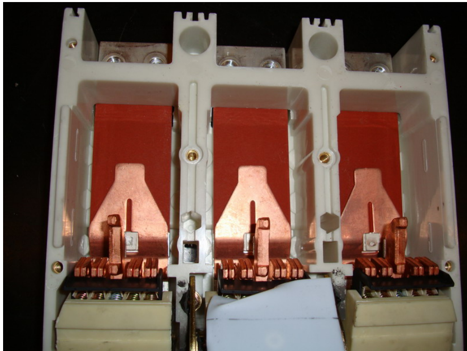
Contact view, after remove the arc chamber
