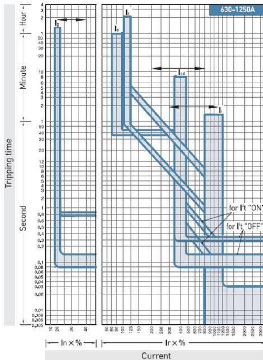
Tripping curve
